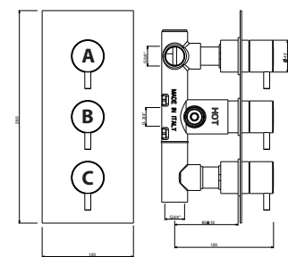
Art. 40990 termostatica thermostatic
