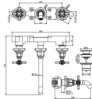
Art. 2321 vitone ceramico ceramic headwork
